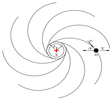
Figure 1: The movement of light aerodynamic configuration of the atom.
